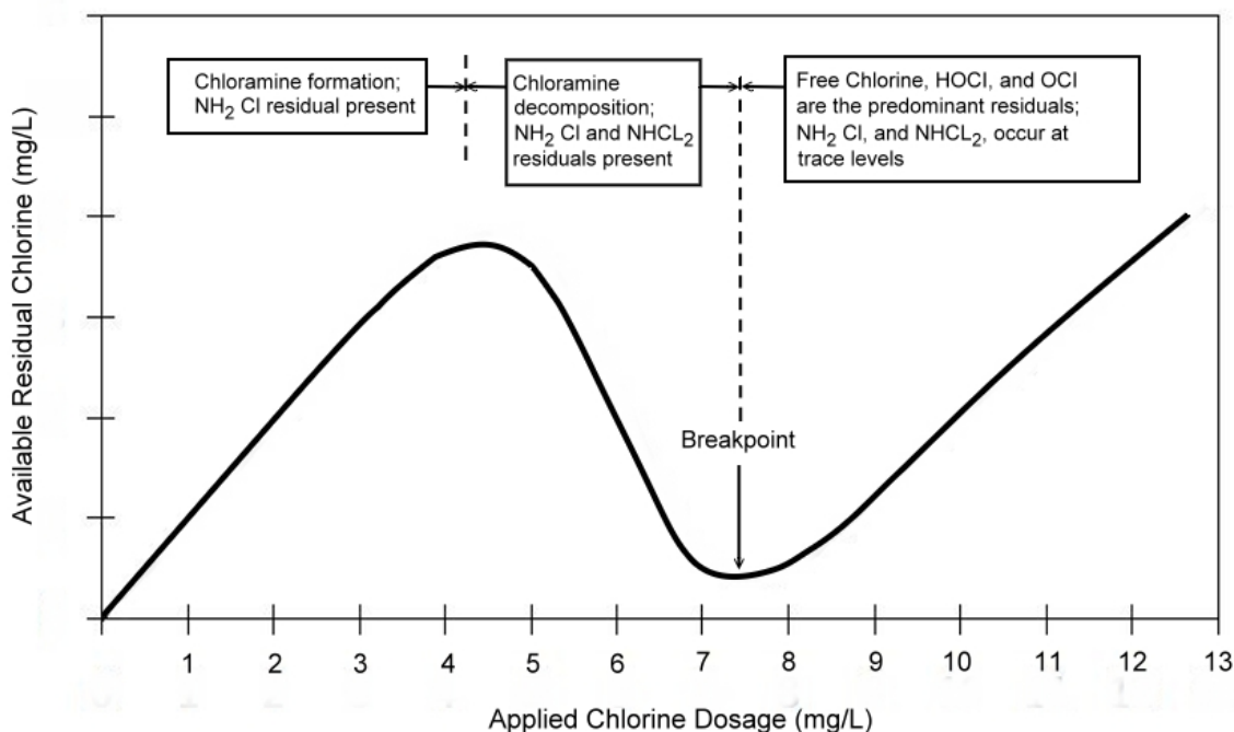
Theoretical breakpoint curve showing increasing amounts of chlorine added to a fixed amount of ammonia.
