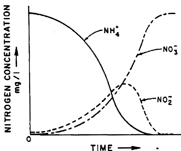
Figure 2. Schematic of nitrogen transformations during noninhibited nitrification, batch experiment.
