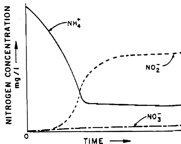
Figure 3. Schematic of nitrification with inhibition of nitrite oxidation, batch experiment.
