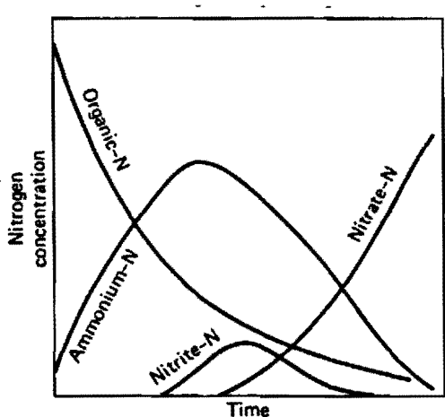
Figure 1. Nitrogen Conversion in a Polluted Stream. (After Sawyer and McCarty, 1967.)
